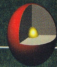
Hydrogen nucleus
